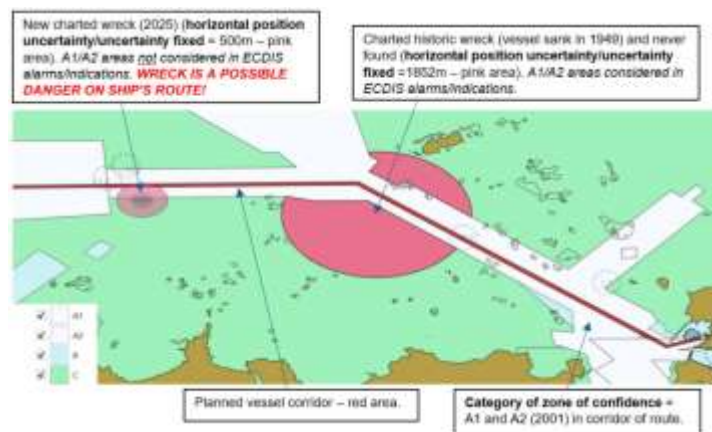
Figure 13-2 – New wreck, possible danger on ships planned route
